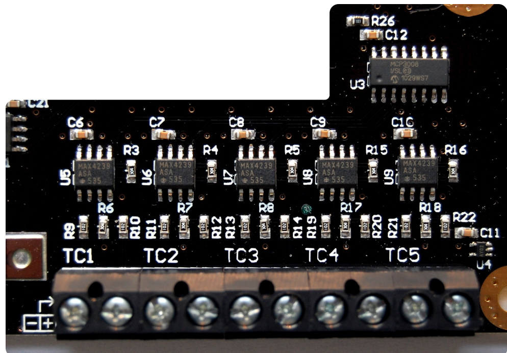
Figure 6: Temperature measurement circuitry
