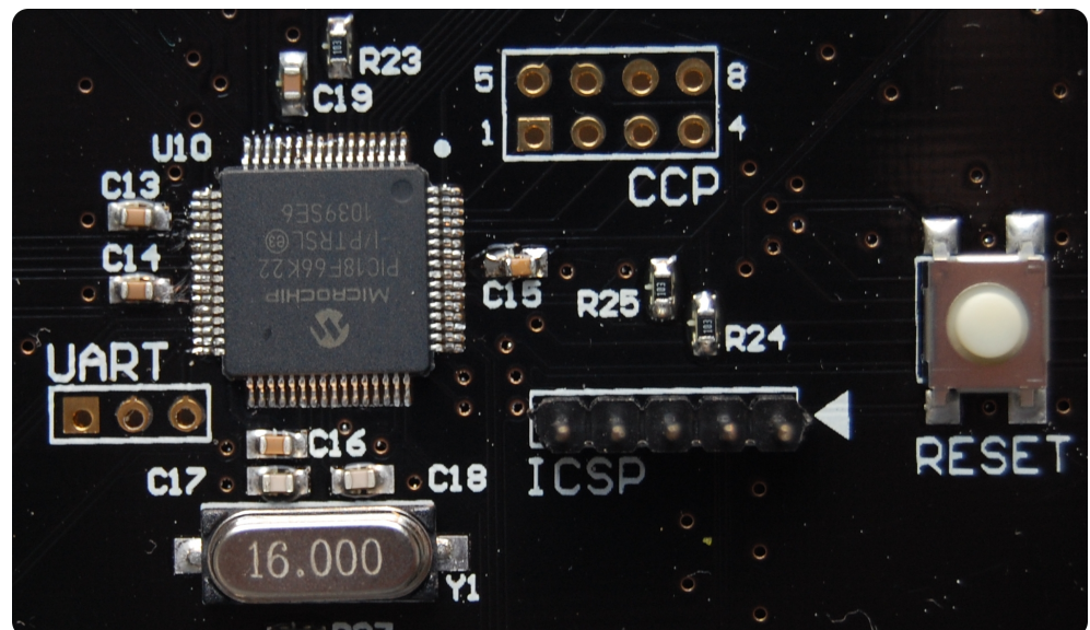
Figure 2: Microcontroller circuitry
