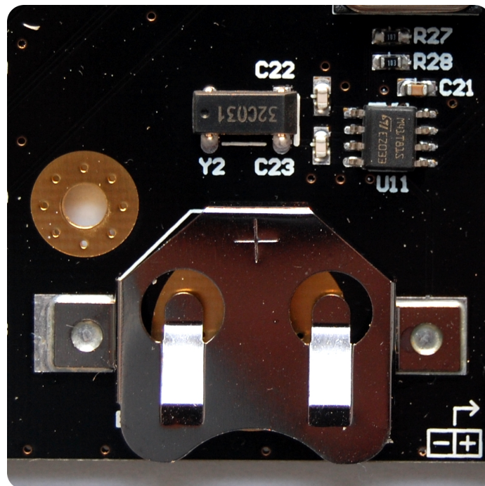
Figure 13: Real Time Clock circuitry
